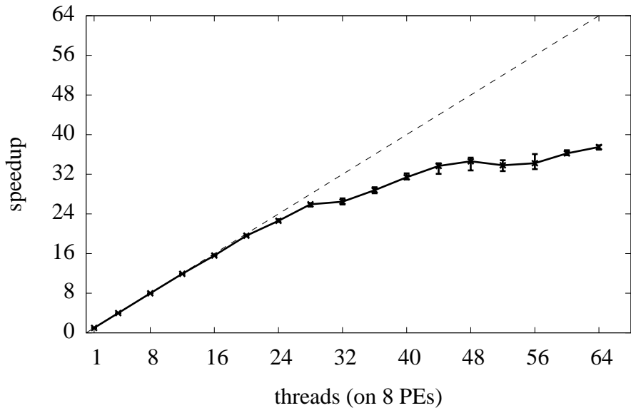
Matrix-matrix multiplication on 1.4Ghz UltraSPARC T2
